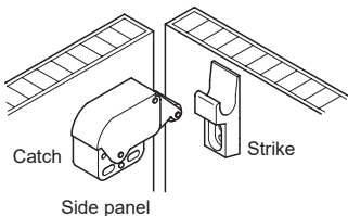
Mounting diagram
